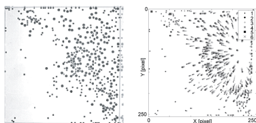
Fig.3 運動粒子群の衝突解析 Fig.3 Collision Analysis of Moving Particles
