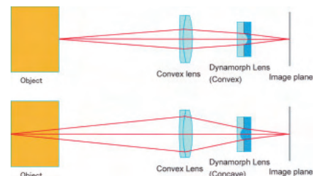
図1 構築した光学系 Figure 1. Schematic diagram of the developed High-Speed Variable-Focus Optical System.
