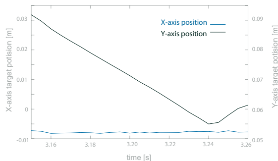
Fig. 10. Time response: target position
