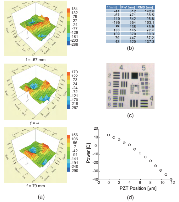
Fig. 3. Optical performance of the prototype [5]: (a) Wavefront-error distribution at the exit pupil of the lens when its focal length f was -67 mm, \infty , and 79 mm. (b) Peak-to-valley (P-V) and root mean square (RMS) wavefront errors. (c) A photograph of a USAF 1951 chart captured by a CMOS imager through the prototype with f = 80 mm and object-side numerical aperture of 0.045. (d) Refractive power (inverse of focal length, D = 1/\text{m} ) versus the displacement of the actuator.
