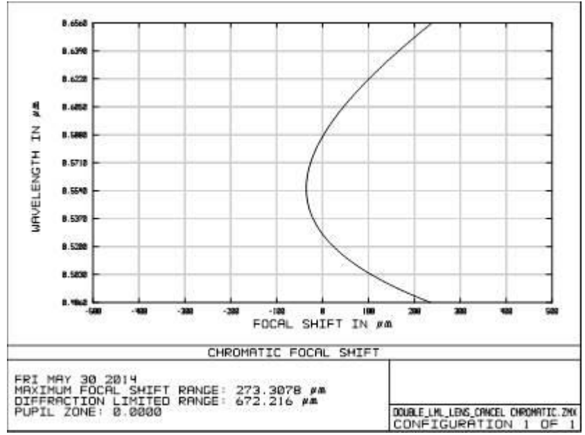
(Right) Chromatic focal shift of Doublet Singlet.
