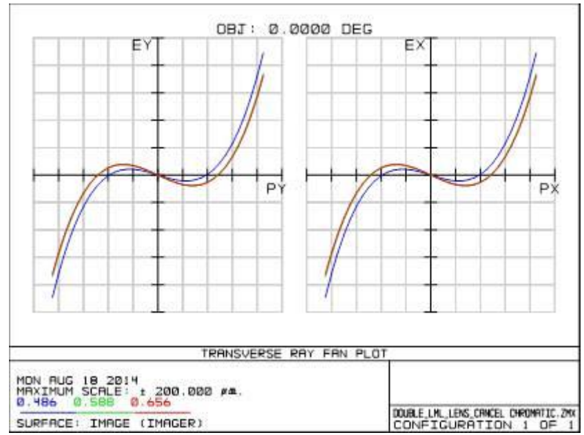
(Right) Ray fan of Doublet Singlet.
