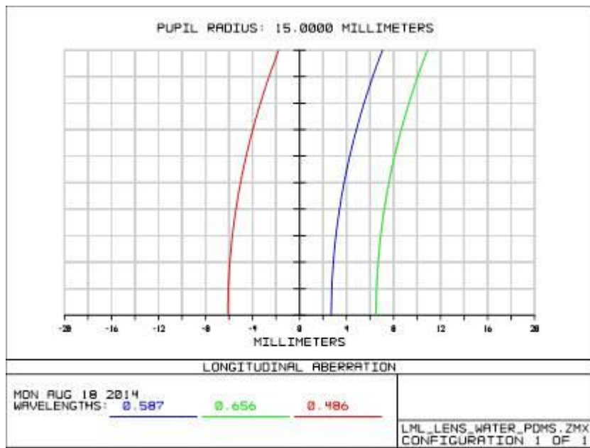
Figure 3. (Left) Longitudinal aberration of Adaptive Singlet.
