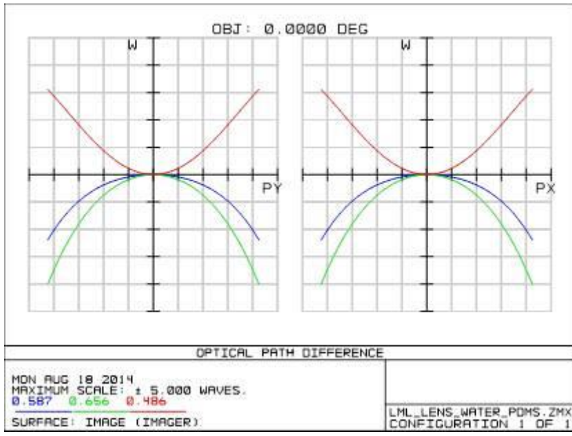
Figure 1. (Left) Opd fan of Adaptive Singlet.
