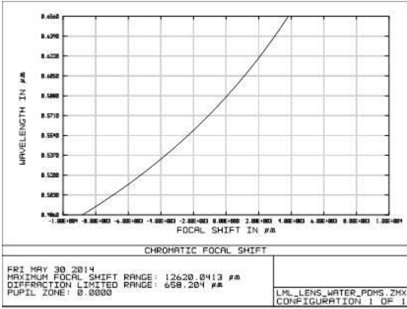
Figure 4. (Left) Chromatic focal shift of Adaptive Singlet.
