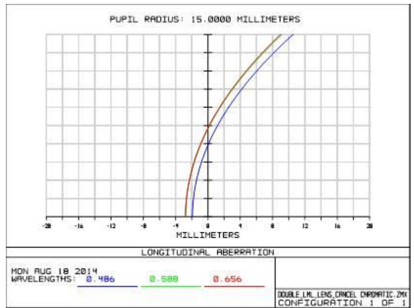
(Right) Longitudinal aberration of Doublet Singlet.
