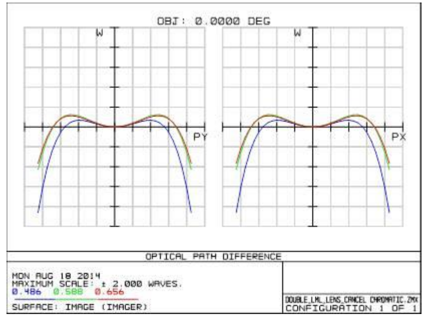
(Right) Opd fan of Doublet Singlet.
