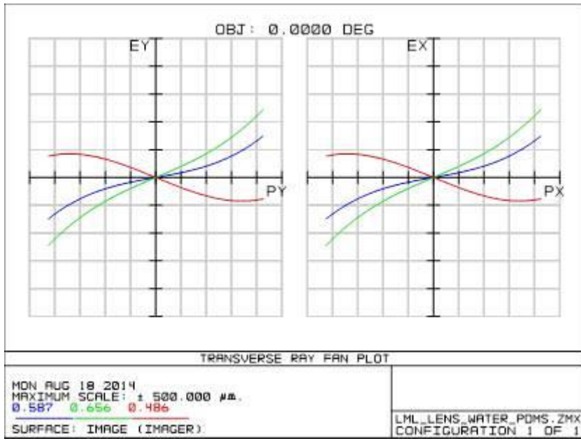
Figure 2. (Left) Ray fan of Adaptive Singlet.
