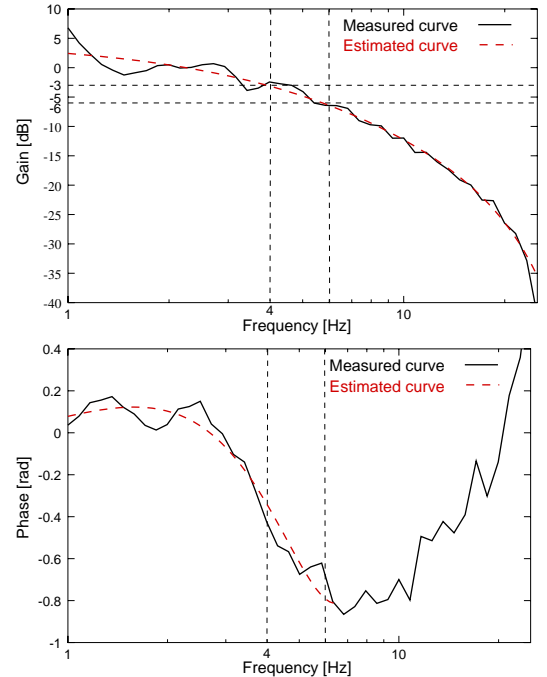
Fig. 4 Frequency response
