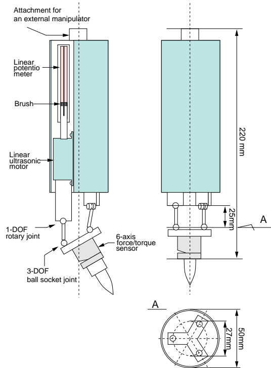
Fig. 1 Mechanism
