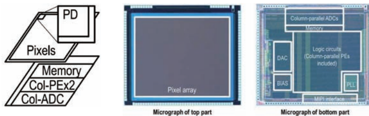
Fig. 1: Vision Chip Architecture and Micrograph*1.
