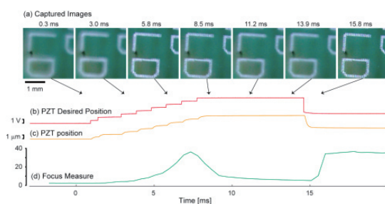
Figure 1. Experimental results for high-speed autofocus ing of an electronic substrate.
