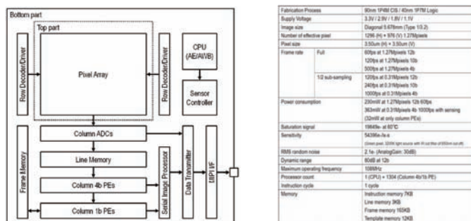
Fig. 2: Block Diagram and Specifications*1.
